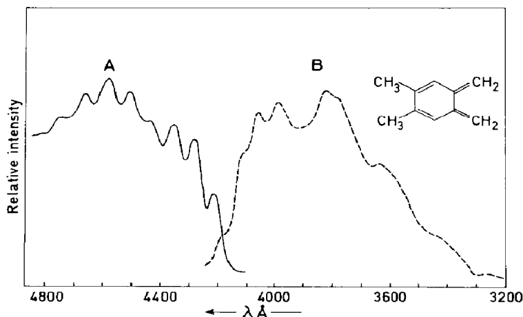
Fig. 4. Electronic spectra of o -durylene produced by photolysis of durene ( C = 10^{-3} M) in n -hexane at 77 K. A, Fluorescence excited by \lambda = 3600 Å radiation; B, excitation spectra of the fluorescence at \lambda = 4750 Å.
