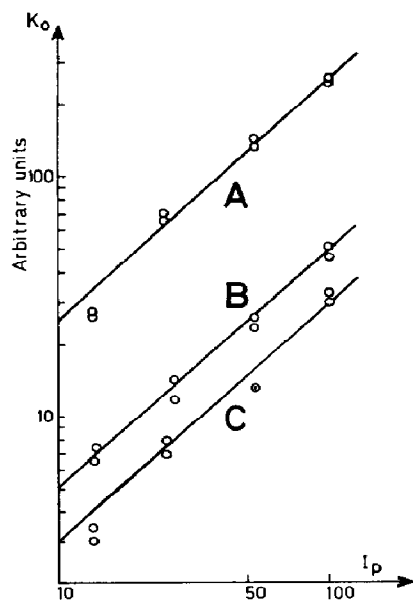
Fig. 2. Photolyzing light intensity I_p dependence of the initial rate K_0 of the photoenol formation in a durene matrix at room temperature from: A, 2,5-dimethylbenzaldehyde; B, 2,4-dimethylbenzaldehyde; C, 2,4,5-trimethylbenzaldehyde.
