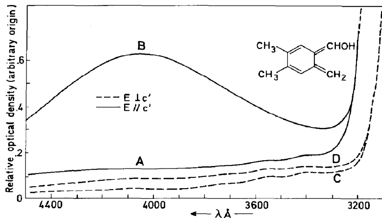
Fig. 1. Polarized absorption spectra of the 2,4,5-trimethylbenzaldehyde photoproduct in durene single crystal at room temperature. Spectra recorded before (A and C) and after (B and D) photolysis at room temperature. The electric vector E of the light beam is polarized along c' (A and B) and perpendicular (C and D) to the durene c' axis.
